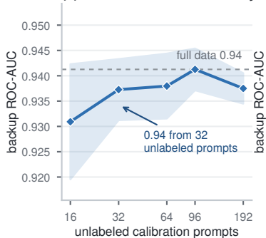
(a) calibration saturates early
