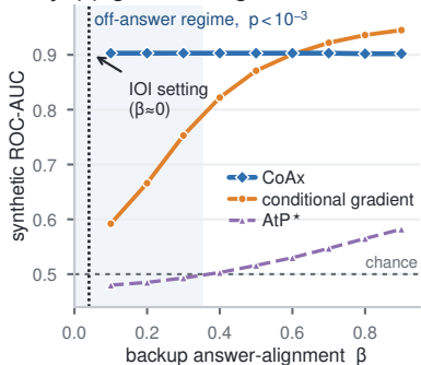
(c) growth is alignment-invariant
